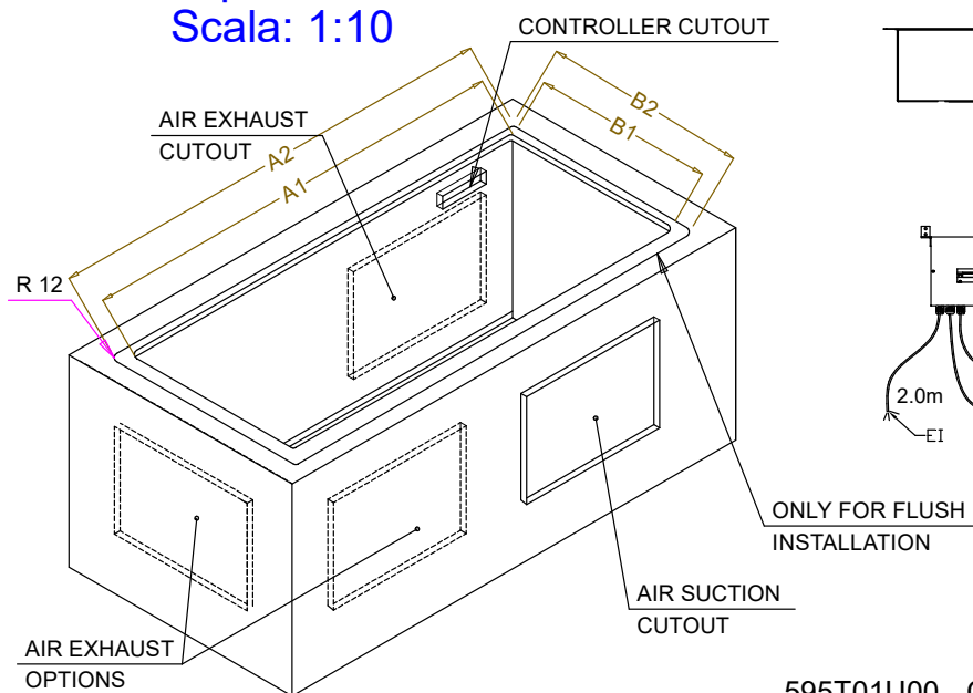
595T01U00 - COLD COMPACT DISPLAY
